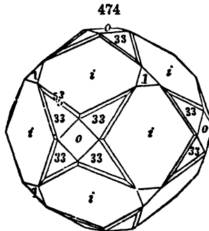
Achmatovsk.
